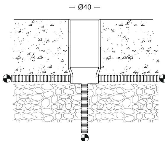
Ground Recessed
